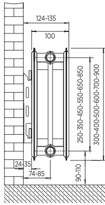
DF Double Panel Double Convactor
