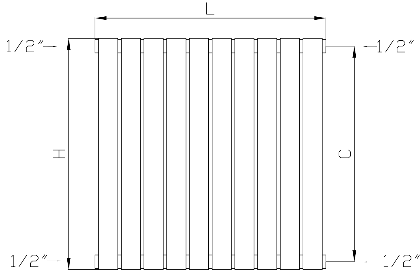
Front View
