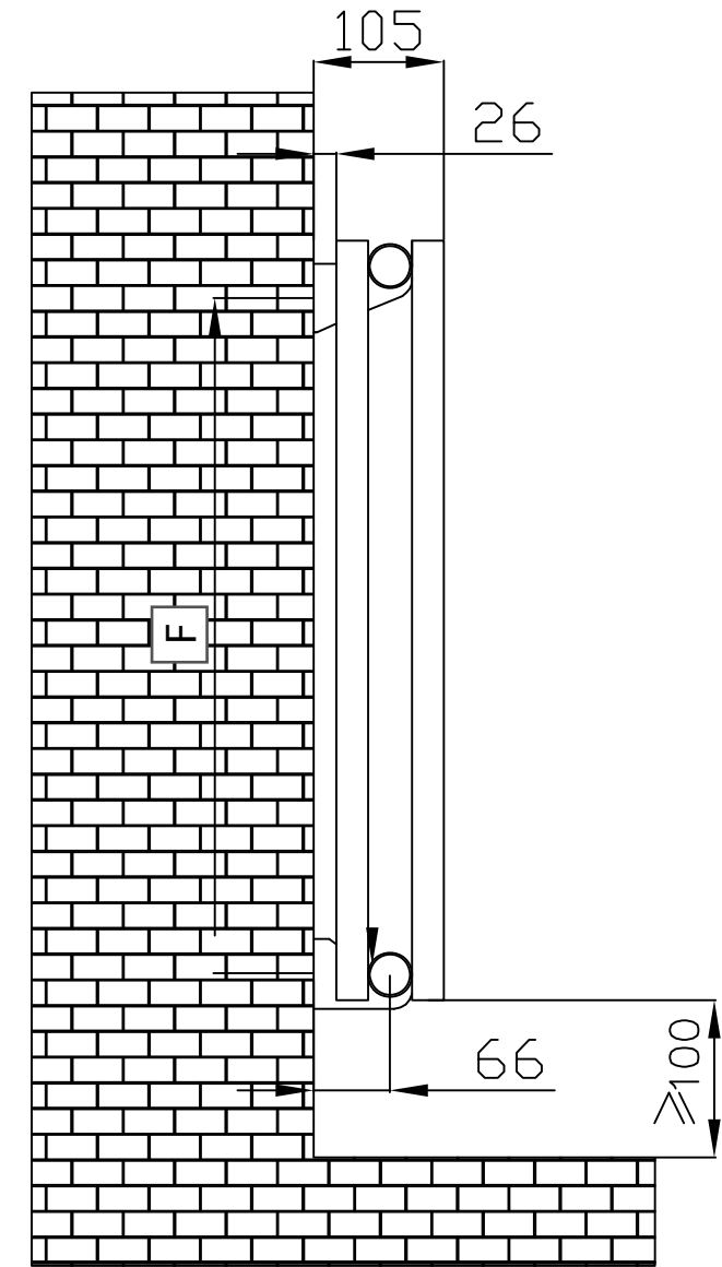
Side View
