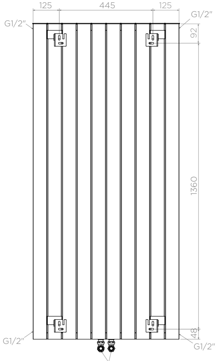
Back View
