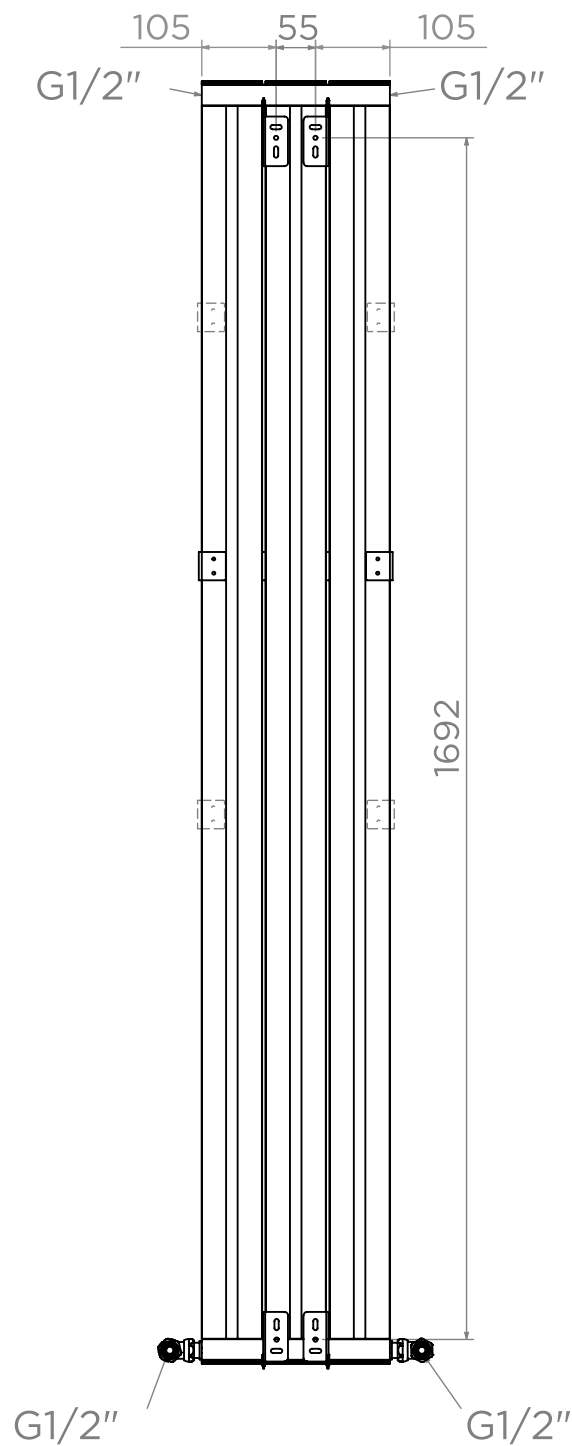
Back View
