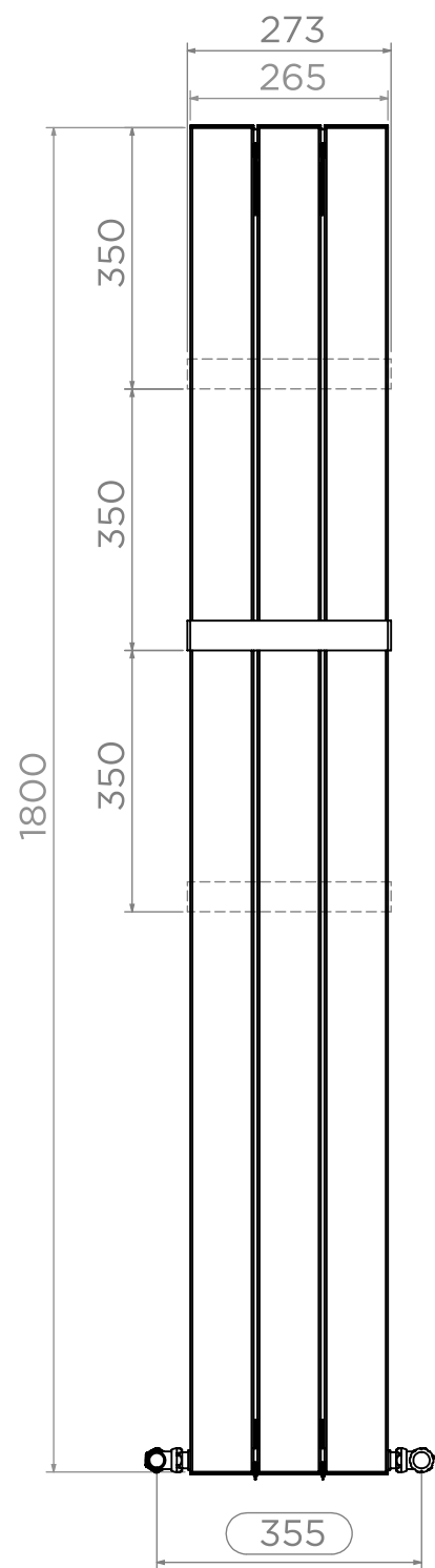
Front View
