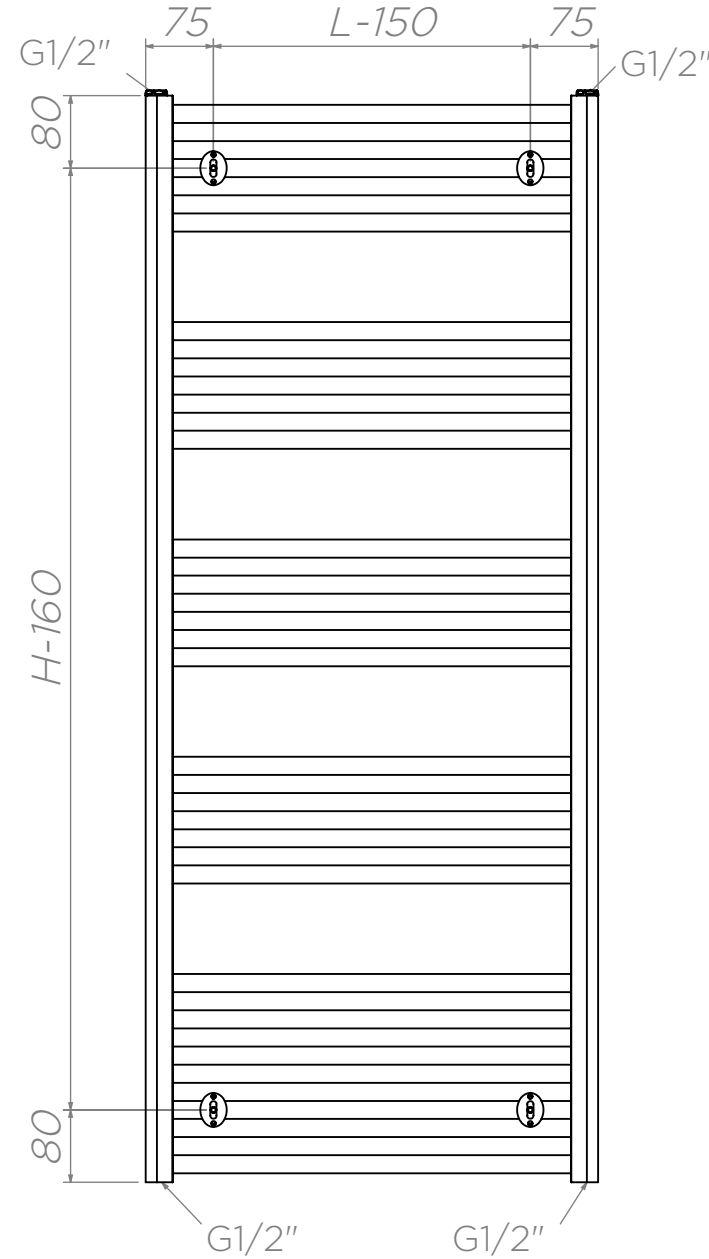
Back View
