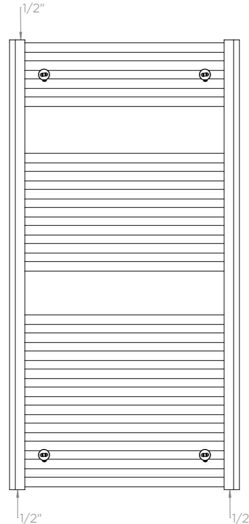
Back View
