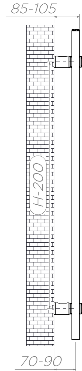
Side View
