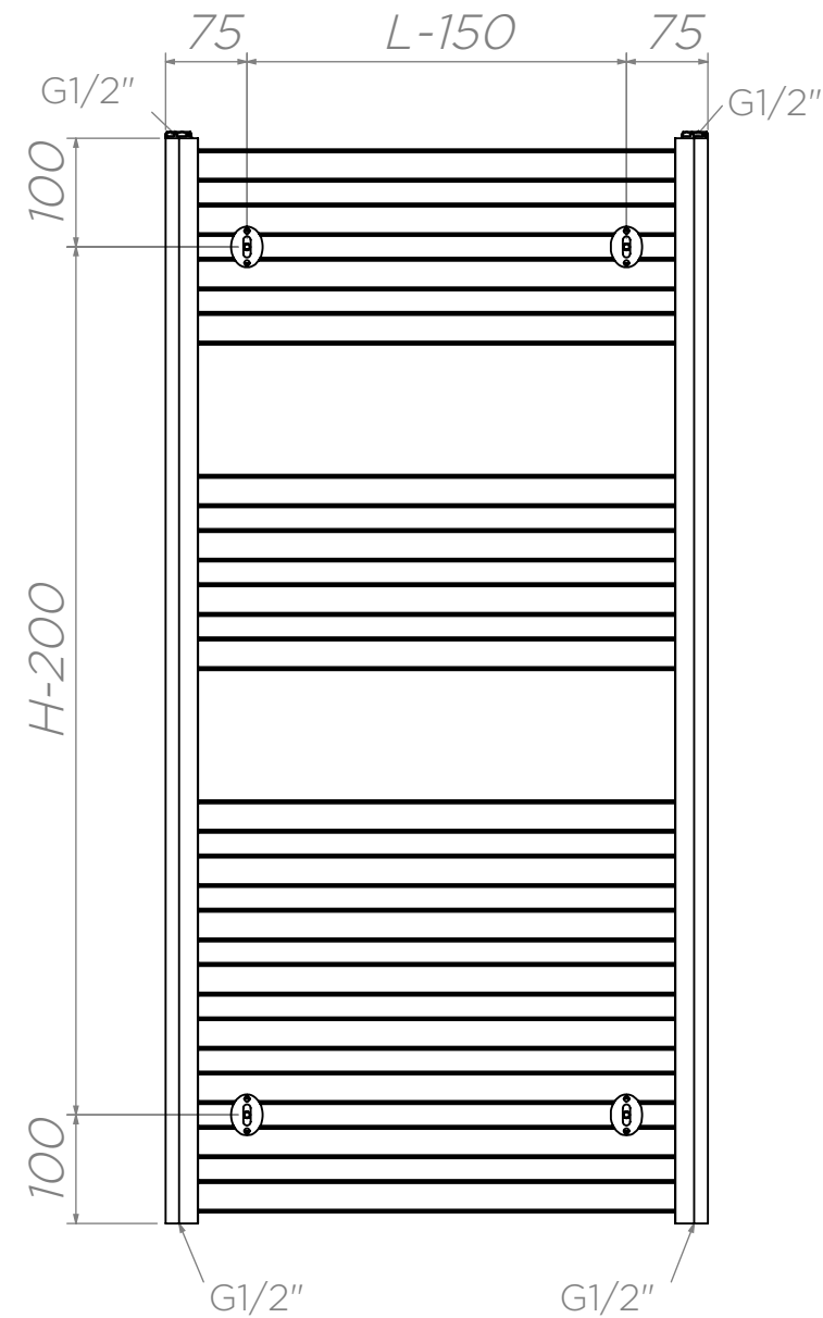
Back View
