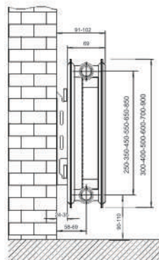
HF DOUBLE PANEL SINGLE CONVECTOR
