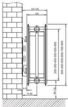
DF DOUBLE PANEL DOUBLE CONVECTOR
