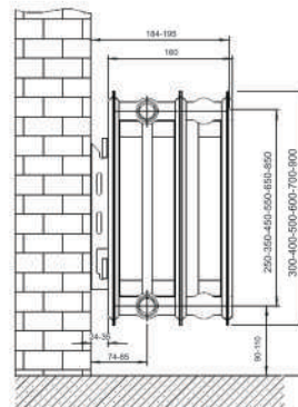
TS TRIPLE PANEL TRIPLE CONVECTOR
