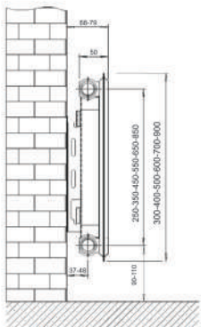
SF SINGLE PANEL SINGLE CONVECTOR
