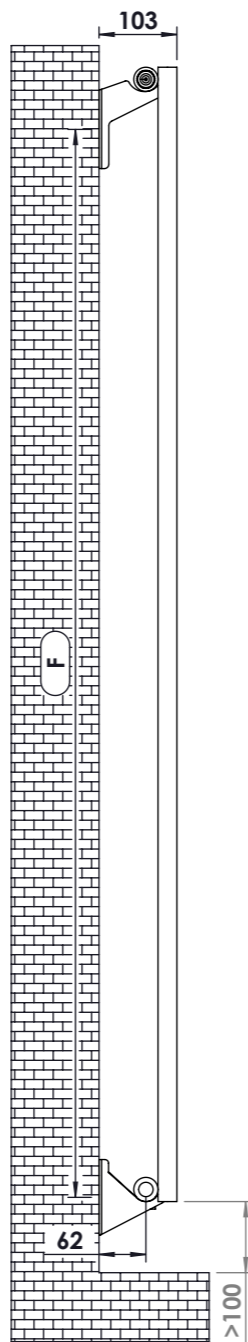
Side View
