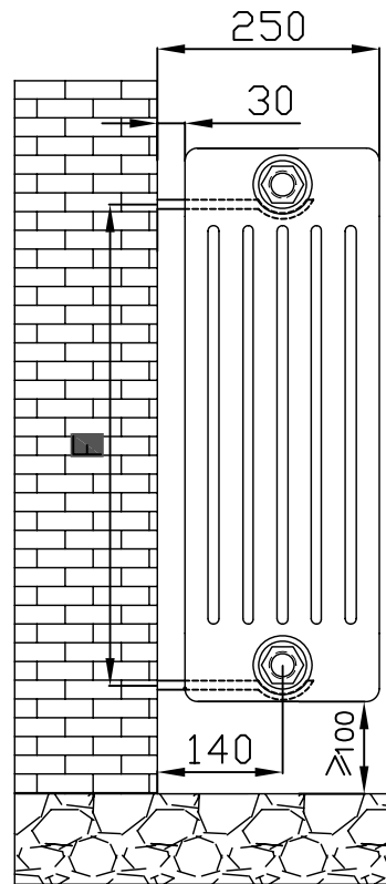
Side View
