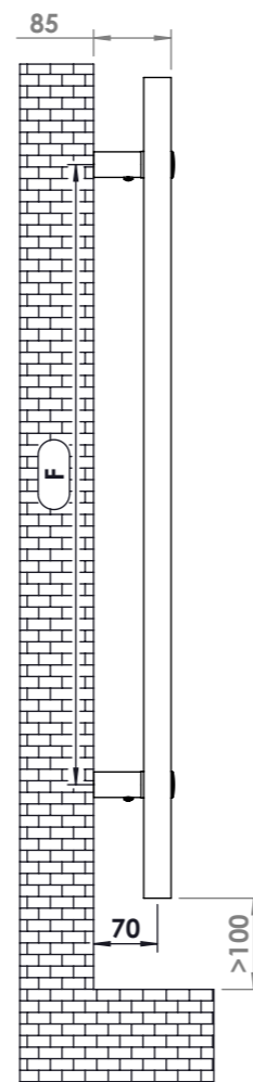
Side View
