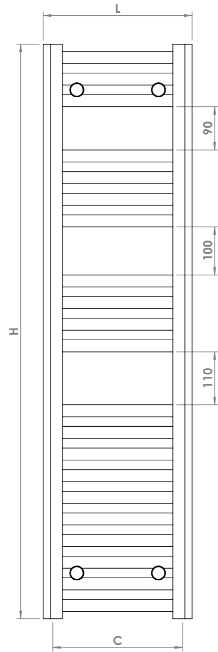
Front View
