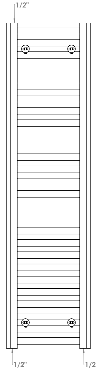
Back View
